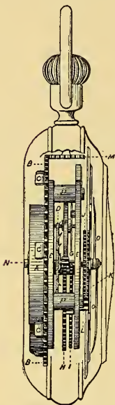
END VIEW.
